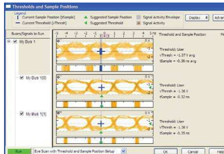
Figure 5. Identify problem signals quickly by viewing eye diagrams across all buses and signals simultaneously.
