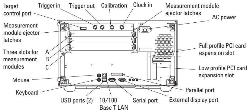
Figure 18. Agilent 16903A back panel
